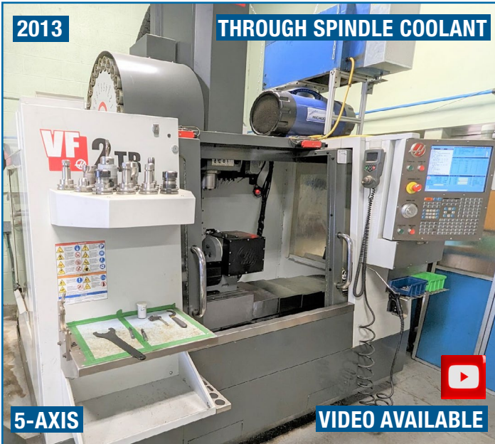
HAAS VF-2TR CNC VERTICAL MACHINING CENTER
